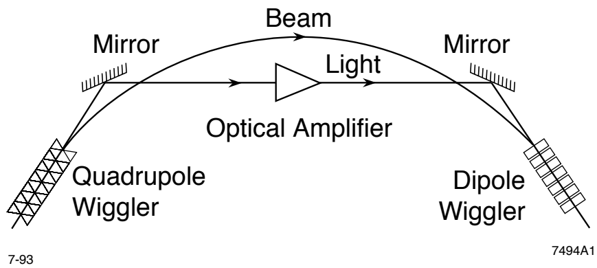
Fig. 1. General layout of the system.
